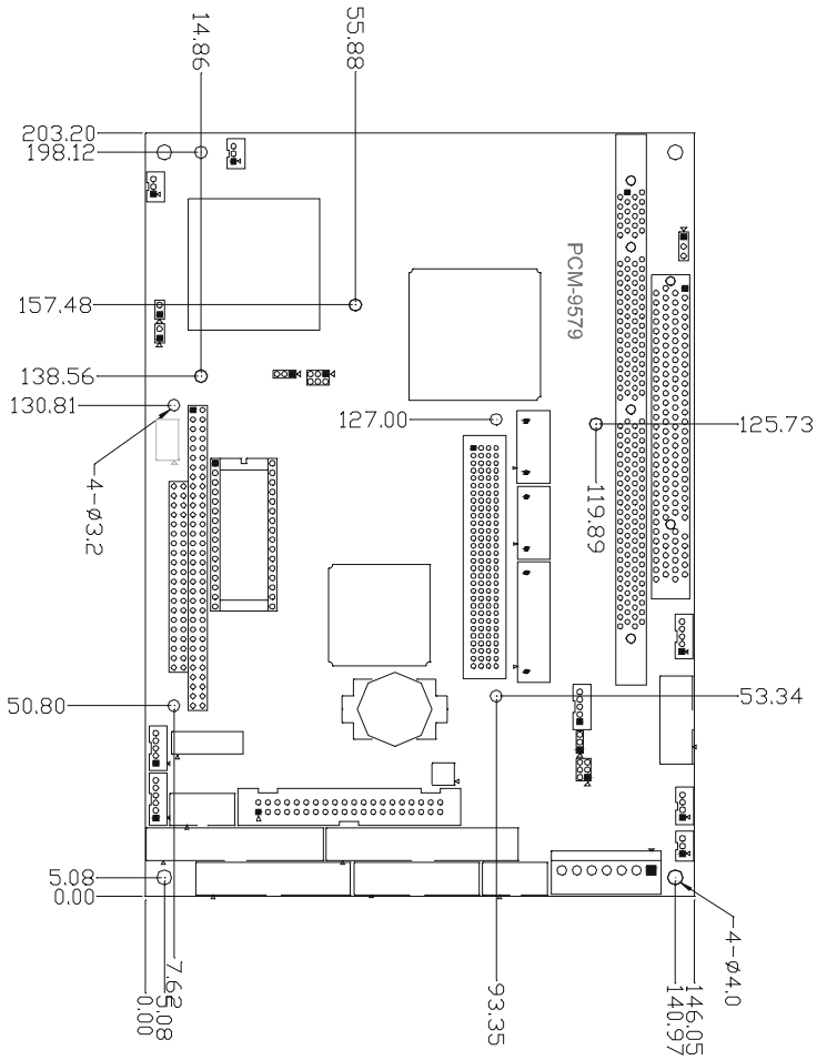
Figure 1.1: Board layout: dimensions
