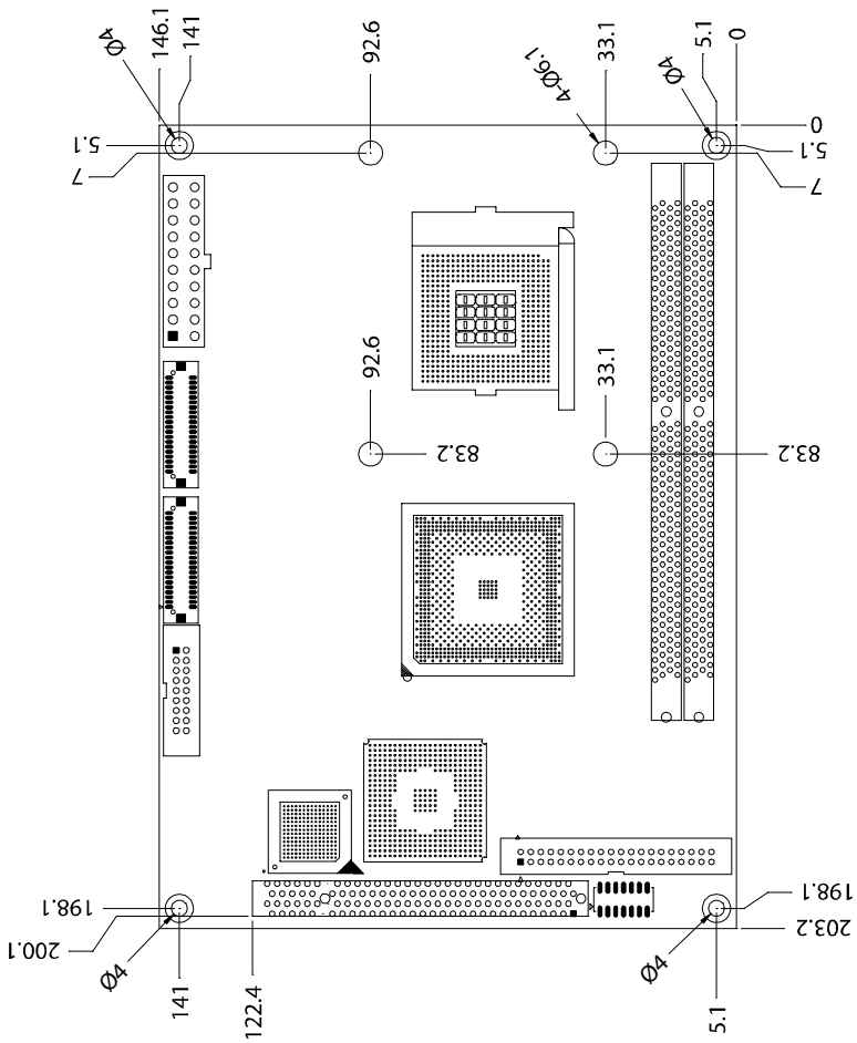
Figure 1.1: Board layout: dimensions
