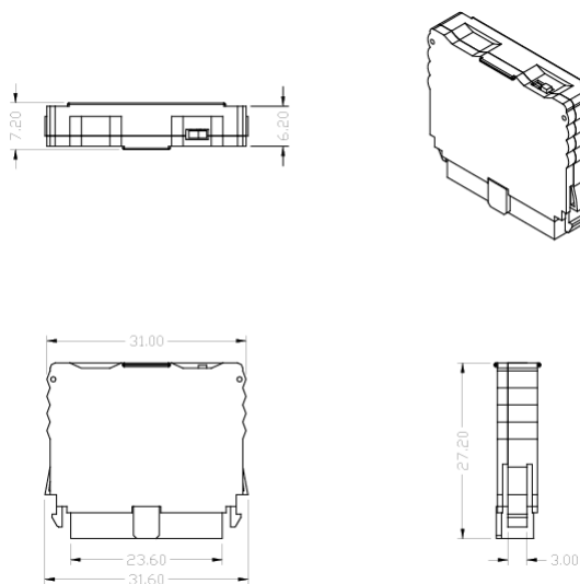
Figure 2.2: Embedded USB Module Type I Form Factor
