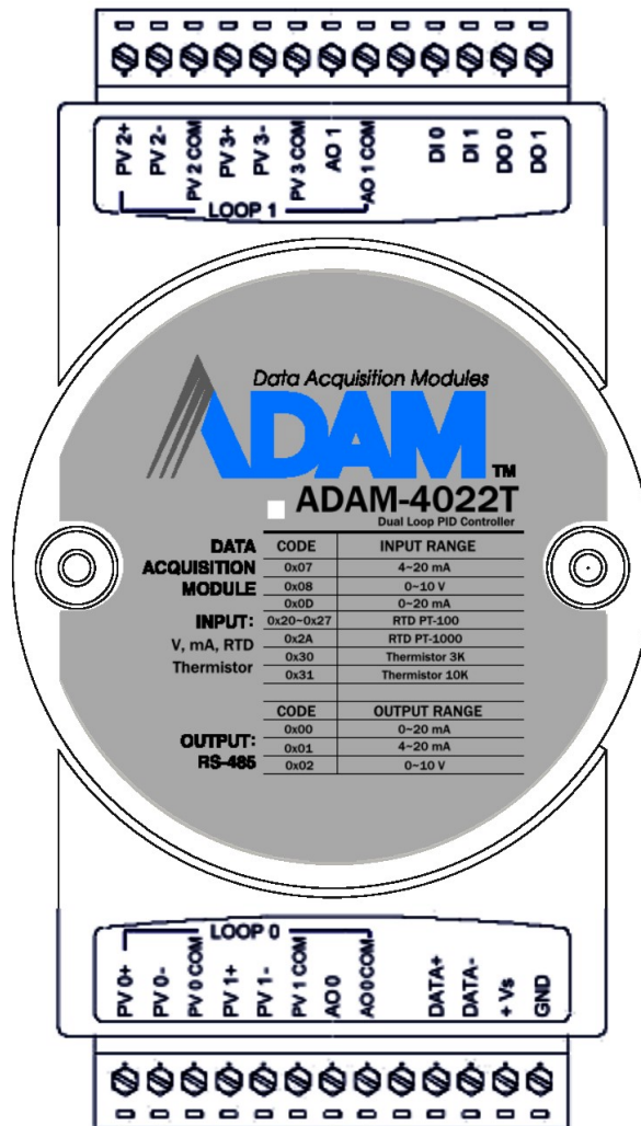
Fig. 7-1 ADAM-4022T Drawing
