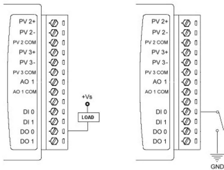
Fig. 7-3 Digital Input/Output Wiring Diagram
