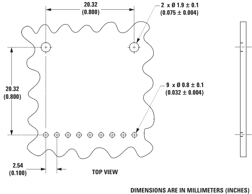
Figure 4. Recommended Board Layout Hole Pattern
