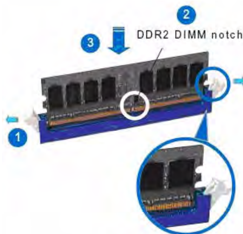
Unlocked retaining clip
