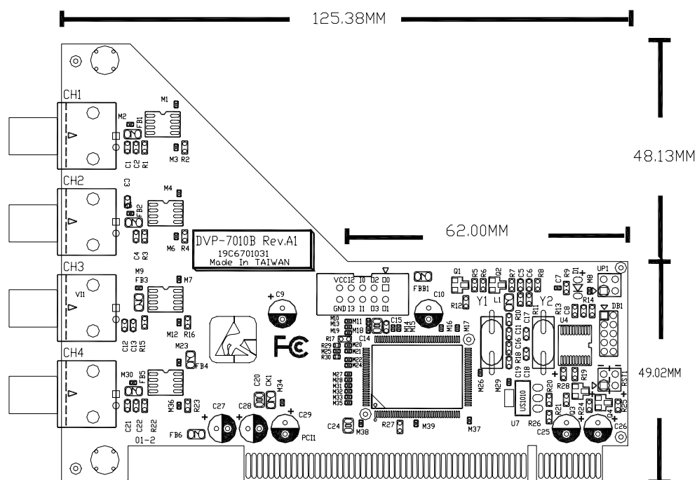
Figure 1.2 Dimensions
