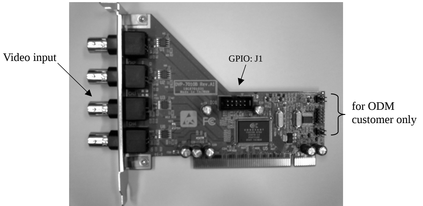
Figure 1.3 connector location
