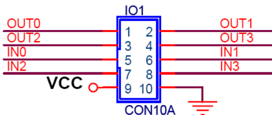
Figure 1.4 GPIO(J1) pin definition
