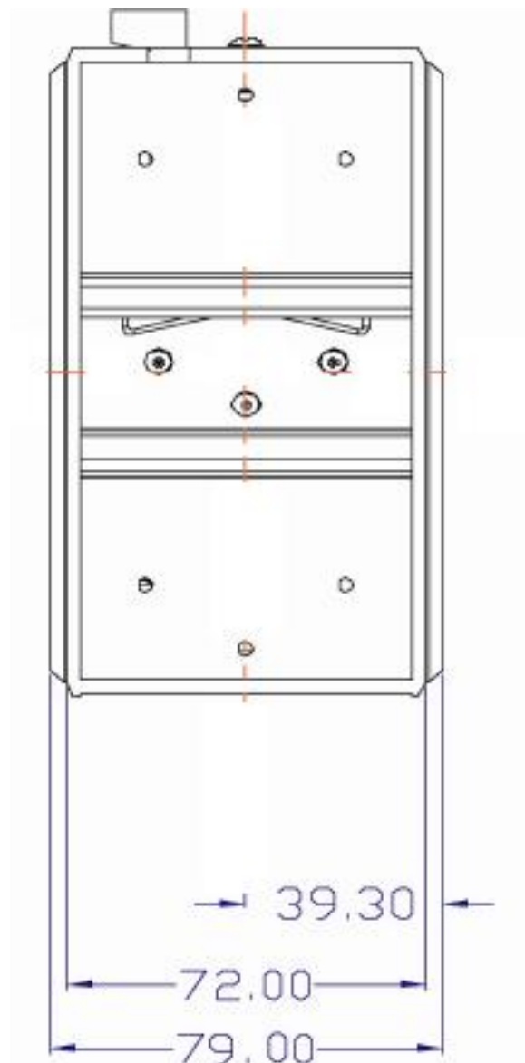
Figure 2.3: Rear View of EKI-7659C
