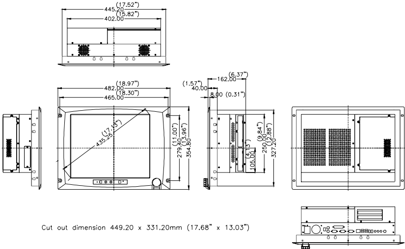
Figure 1.1: IPPC-9171G Dimensions
