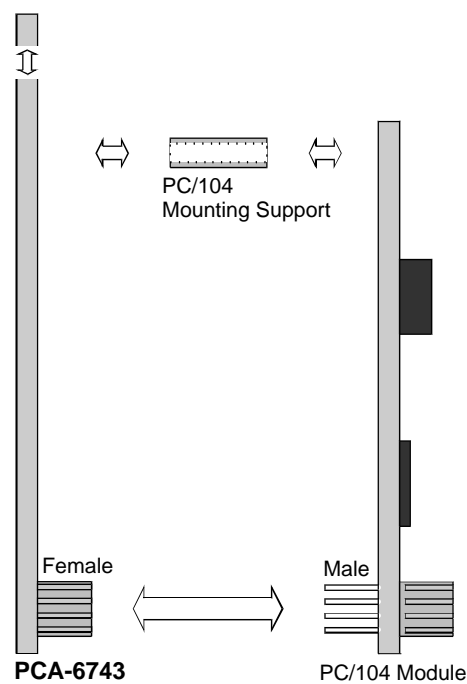
Figure D.1 PC/104 module mounting diagram
