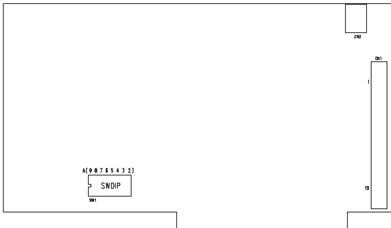
Card connector, jumper and switch locations
