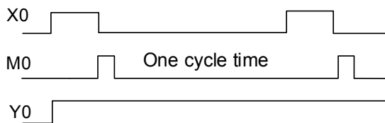
PLF(M0) Timing diagram
