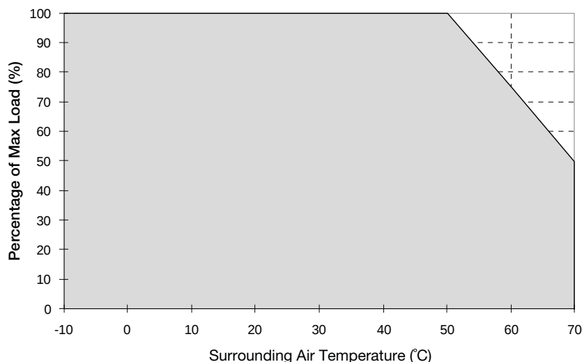
Fig. 1.1 De-rating for Vertical and Horizontal Mounting Orientation > 50°C de-rate power by 2.5% / °C
